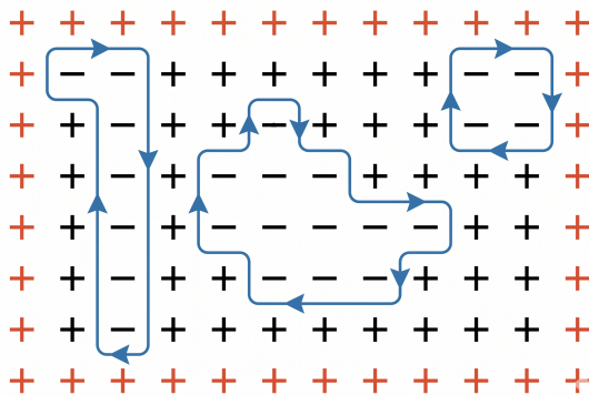
Figure 3.6: Example of configuration with fixed open boundary conditions, where the spins on the boundary are all up (red), and three droplets of flipped spins inside the (blue) oriented domain walls.
