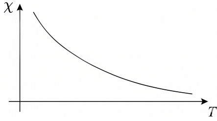
Figure 3.2: Magnetic susceptibility \chi as a function of temperature T at zero external field h = 0 .
