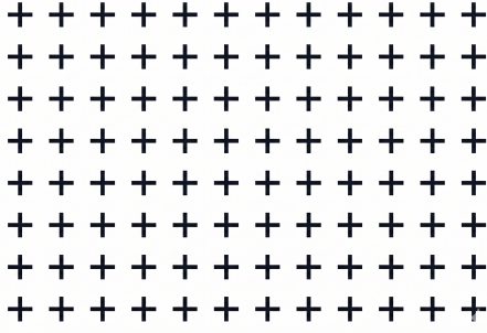
Figure 3.3: Configuration A: no domain walls, fully magnetized.
