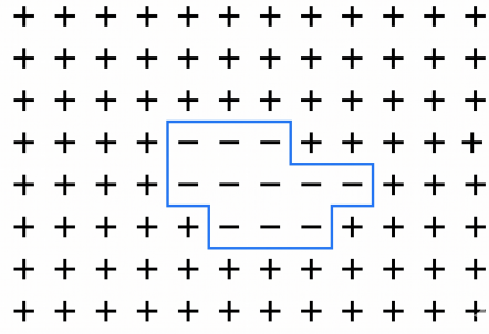
Figure 3.4: Configuration B: one domain wall, with a droplet of flipped spins.
